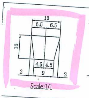
t1.5ガasket詳細
